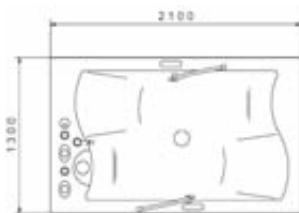
Dimensions Rendezvous
