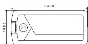
Dimensions Thermo-Spa standard cladding
