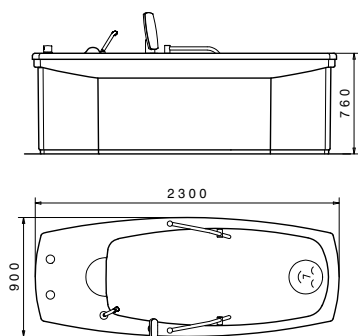
Alpha cladding dimensions
