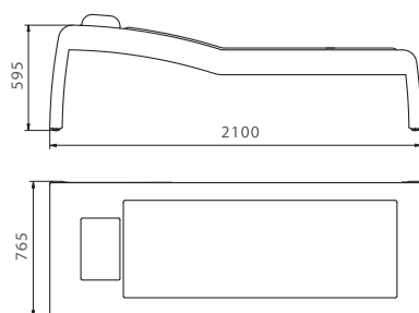
Dimensions Revital Wellness Bed
