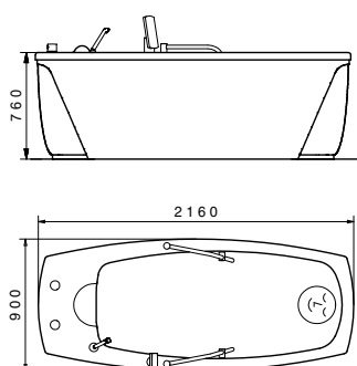
Dimensions Florida 100 California 100 Diane 100
