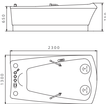
California Twin dimensions
